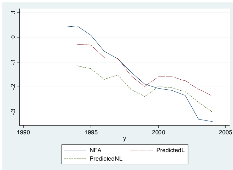
Figure 25. Actual and predicted NFA for Romania
