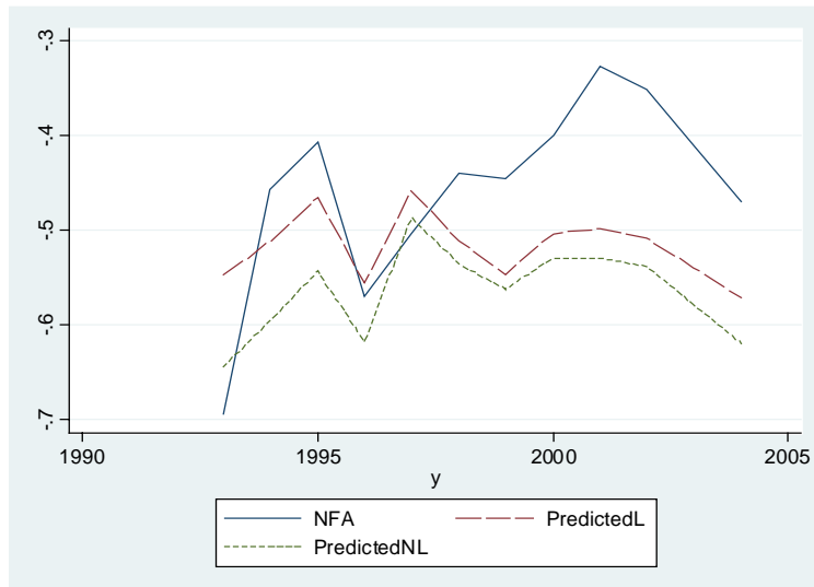
Figure 19. Actual and predicted NFA for Czech Republic
